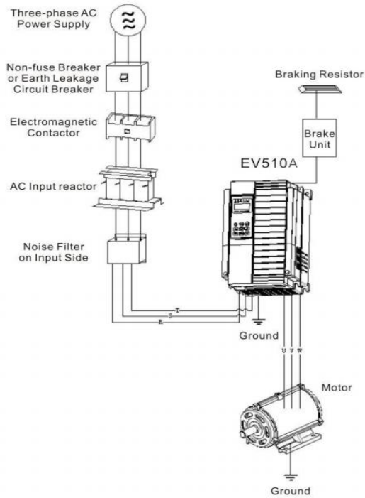
Figure 3-2 Connection to Peripheral Devices
