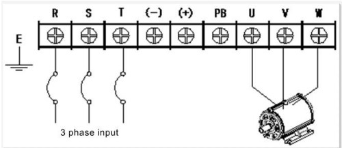
f) The Major Loop Terminal Block Distribution Diagram of 75-110KW.
