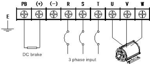
e) The Major Loop Terminal Block Distribution Diagram of 55KW.
