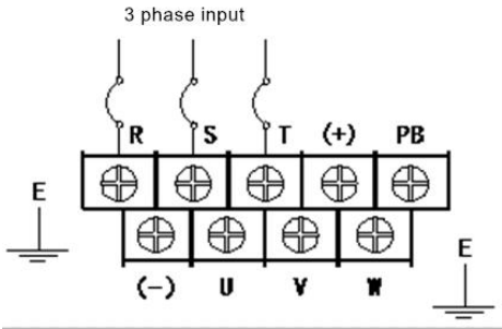
f) The Major Loop Terminal Block Distribution Diagram of 75-110KW.
