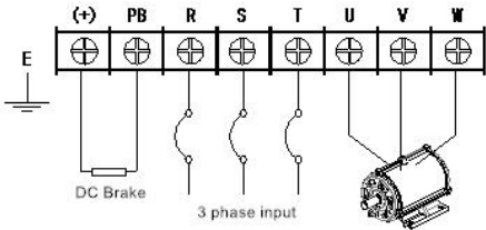
d) The Major Loop Terminal Block Distribution Diagram of 37KW-45KW.
