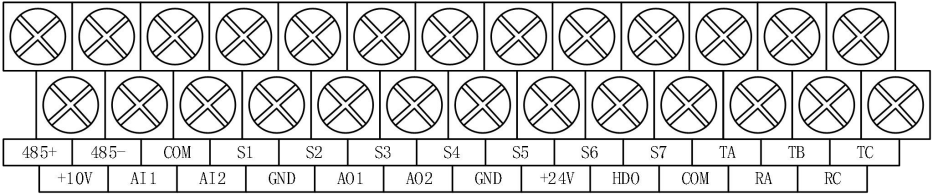
Fig. 3-3 Control Loop Wiring Terminal Diagram
