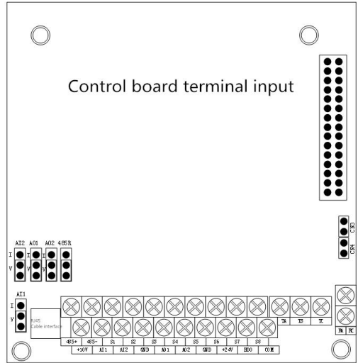
Figure 3-4 Control terminal shows
